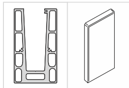
SBRL-18 PROFILE
