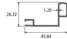
MESH TRACK SECTION NO. : 955369 Weight / Mtr : 0.355
