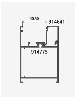
DGU CLIP SECTION NO. : 914641 Weight / Mtr : 0.230
