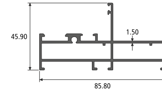
BIG FRAME SECTION NO. : 914756 Weight / Mtr : 1.185
