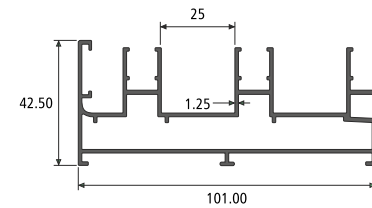
3 TRACK SECTION NO. : 955389 Weight / Mtr : 1.240
