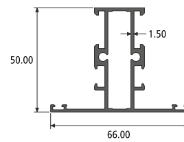
MULLION SECTION NO. : 914352 Weight / Mtr : 1.015
