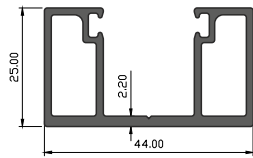
FIXED PROFILE
