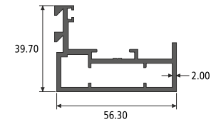
SHUTTER SECTION NO. : 992097 Weight / Mtr : 1.106
