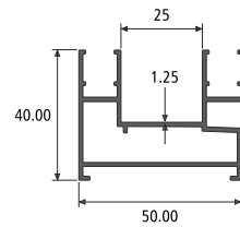
2 TRACK SECTION NO. : 955388 Weight / Mtr : 0.795
