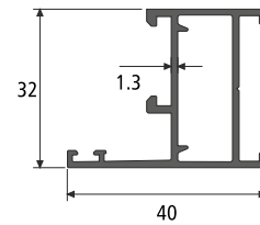
FRAME SECTION NO. : 745611 Weight / Mtr : 0.449
