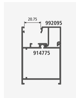
LAMINATED GLASS CLIP SECTION NO. : 992095 Weight / Mtr : 0.288
