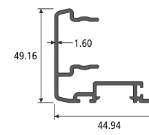
INTERLOCK SECTION NO. : 992312 Weight / Mtr : 0.693
