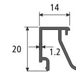
SGU CLIP SECTION NO. : 746509 Weight / Mtr : 0.202
