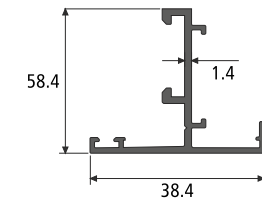
INVERSION PROFILE SECTION NO. : 746510 Weight / Mtr : 0.369
