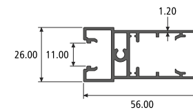
3 TRACK SECTION NO. : 992011 Weight / Mtr : 1.450
