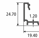
DGU CLIP SECTION NO. : 992036 Weight / Mtr : 0.193
