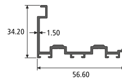
DOOR BOTTOM ADAPTOR SECTION NO. : 992208 Weight / Mtr : 0.526
