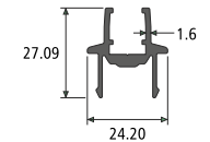
MATING SECTION NO. : 992088 Weight / Mtr : 0.396
