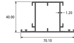
BIG SHUTTER SECTION NO. : 914891 Weight / Mtr : 0.755
