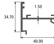
INVERSION SECTION NO. : 819014 Weight / Mtr : 0.433
