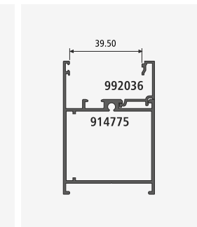
DGU CLIP SECTION NO. : 992036 Weight / Mtr : 0.193
