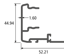
INTERLOCK SECTION NO. : 955110 Weight / Mtr : 0.689
