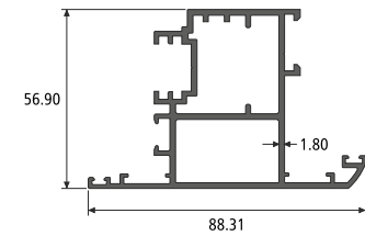
SHUTTER SECTION NO. : 992166 Weight / Mtr : 1.623
