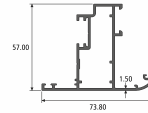
SHUTTER SECTION NO. : 992178 Weight / Mtr : 1.100
