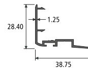
INTERLOCK SECTION NO. : 914038 Weight / Mtr : 0.273
