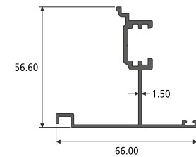
FLYING MULLION SECTION NO. : 914797 Weight / Mtr : 0.707
