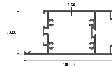
DOOR BOTTOM SECTION NO. : 914777 Weight / Mtr : 1.766
