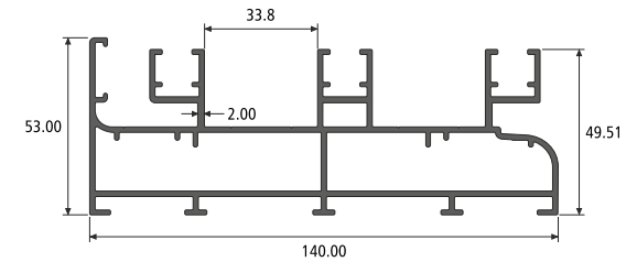
3 TRACK WITH LEG SECTION NO. : 551016 Weight / Mtr : 2.688
