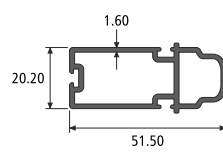
MATING PROFILE FRONT FITTED COUNTER PLATE SECTION NO. : 817072 Weight / Mtr : 0.720
