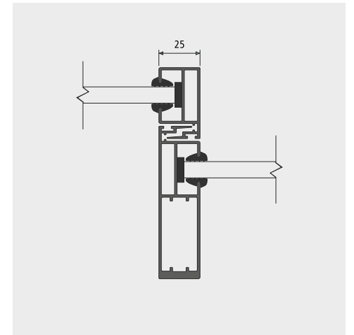
37mm SLEEK INTERLOCK
