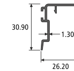
INTERLOCK SECTION NO. : 551025 Weight / Mtr : 0.230
