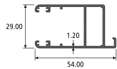
MOSQUITO SHUTTER SECTION NO. : 914698 Weight / Mtr : 0.617
