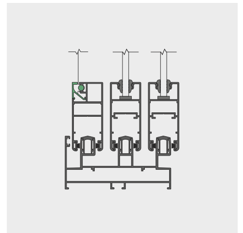
29mm THREE TRACK WITH MOSQUITO
