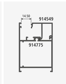
SGU CLIP SECTION NO. : 914549 Weight / Mtr : 0.305
