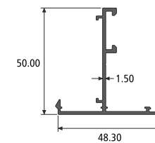
INVERSION SECTION NO. : 914564 Weight / Mtr : 0.508
