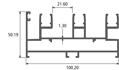
3 TRACK WITH LEG SECTION NO. : 551009 Weight / Mtr : 1.969
