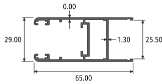
DGU SHUTTER SECTION NO. : 914897 Weight / Mtr : 0.796
