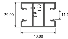
MIDDLE SECTION NO. : 817032 Weight / Mtr : 0.672
