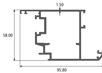
INSIDE OP. SHUTTER SECTION NO. : 992109 Weight / Mtr : 1.540
