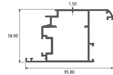
INSIDE OP. SHUTTER SECTION NO. : 992109 Weight / Mtr : 1.540
