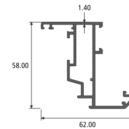
INSIDE OP. SHUTTER SECTION NO. : 914520 Weight / Mtr : 0.955
