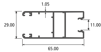
MOSQUITO SHUTTER LIGHT SECTION NO. : 914900 Weight / Mtr : 0.705
