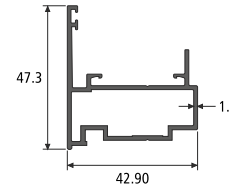
FLING MULLION SECTION NO. : 819002 Weight / Mtr : 0.662
