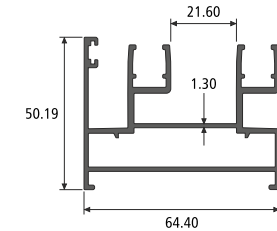
2 TRACK WITH LEG SECTION NO. : 812520 Weight / Mtr : 1.325
