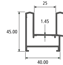
2 TRACK SECTION NO. : 914036 Weight / Mtr : 0.873
