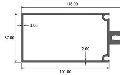
MULLION SECTION NO. : 551026 Weight / Mtr : 2.173
