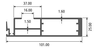
SLEEK REINFORCEMENT INTERLOCK SECTION NO. : 812859 Weight / Mtr : 1.472
