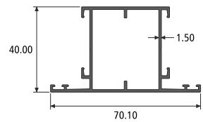
BIG SHUTTER SECTION NO. : 819013 Weight / Mtr : 0.867
