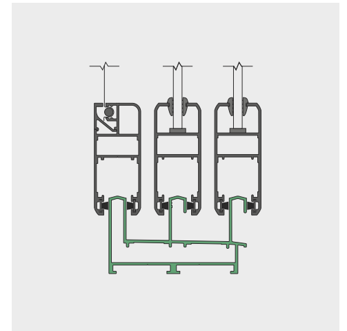
27mm THREE TRACK WITH MOSQUITO
