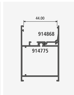
DGU CLIP SECTION NO. : 914868 Weight / Mtr : 0.185
