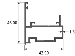
FLYING MULLION SECTION NO. : 819002 Weight / Mtr : 0.662
