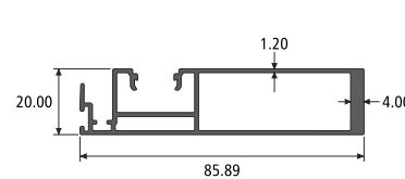
REINFORCEMENT INTERLOCK SECTION NO. : 992268 Weight / Mtr : 0.975
