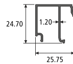
LAMINATED GLASS CLIP SECTION NO. : 992095 Weight / Mtr : 0.288
