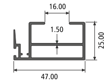
SLEEK INTERLOCK SECTION NO. : 992326 Weight / Mtr : 0.676
