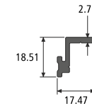
TOGGLE SECTION NO. : 968039 Weight / Mtr : 0.240
