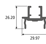
MATING PROFILE INSERTED COUNTER PLATE SECTION NO. : 992148 Weight / Mtr : 0.478
