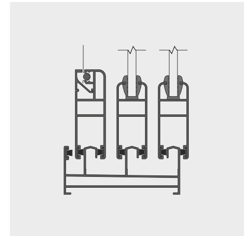
22mm THREE TRACK WITH MOSQUITO NET
