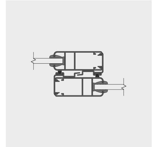
22mm INTERLOCK
