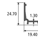
DGU CLIP SECTION NO. : 914868 Weight / Mtr : 0.185
