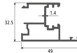
FLYING MULLION SECTION NO. : 819082 Weight / Mtr : 0.623
