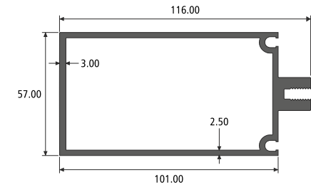
MULLION SECTION NO. : 551027 Weight / Mtr : 2.641
