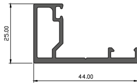
BOTTOM PROFILE
