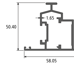
ADAPTOR SECTION NO. : 992165 Weight / Mtr : 1.072
