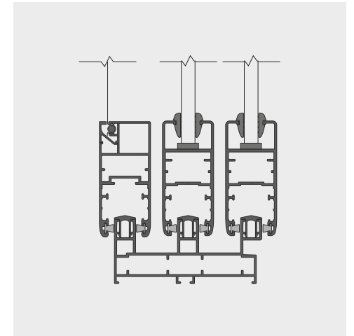
37mm FLYMESH
