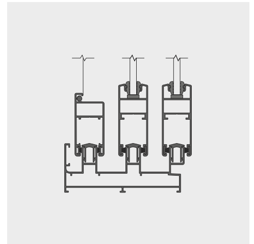
25mm THREE TRACK WITH MOSQUITO
