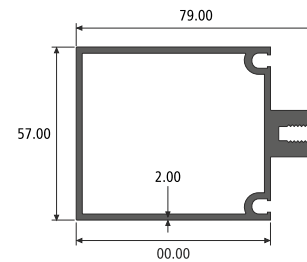
TRANSOM SECTION NO. : 812957 Weight / Mtr : 1.787
