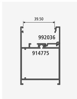
DGU CLIP SECTION NO. : 992036 Weight / Mtr : 0.193
