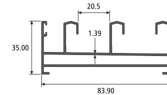
3 TRACK SECTION NO. : 551024 Weight / Mtr : 1.130
