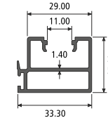
SLEEK INTERLOCK SECTION NO. : 992324 Weight / Mtr : 0.524
