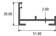
FRAME SECTION NO. : 992098 Weight / Mtr : 0.616
