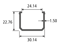
LAMINATED GLASS ADAPTOR SECTION NO. : 992087 Weight / Mtr : 0.297
