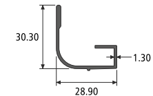
RAIN TRACK SECTION NO. : 914519 Weight / Mtr : 0.283
