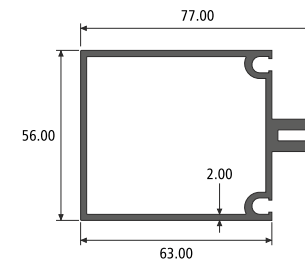
TRANSOM SECTION NO. : 812958 Weight / Mtr : 1.591
