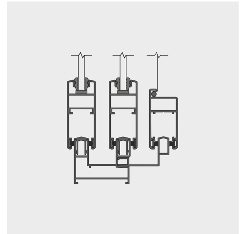
25mm MESH TRACK
