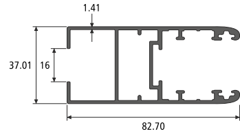
SGU SHUTTER SECTION NO. : 914668 Weight / Mtr : 1.335
