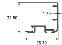
MOSQUITO INTERLOCK SECTION NO. : 955368 Weight / Mtr : 0.310
