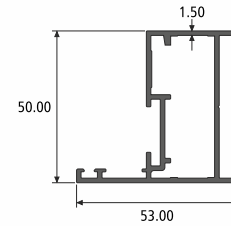
FRAME SECTION NO. : 992177 Weight / Mtr : 0.882
