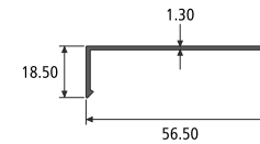
COVER CAP SECTION NO. : 812960 Weight / Mtr : 0.321
