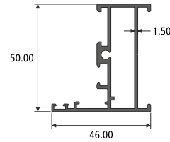
FRAME SECTION NO. : 914351 Weight / Mtr : 0.818
