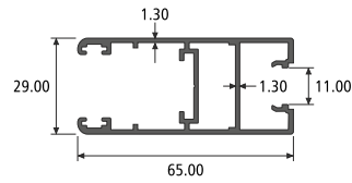
SGU SHUTTER SECTION NO. : 914405 Weight / Mtr : 0.890
