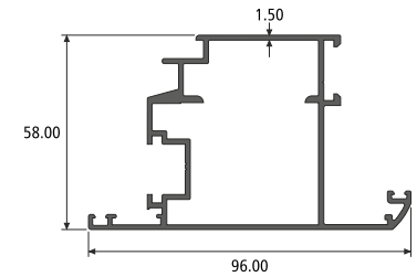
OUTSIDE OP. SHUTTER (MULTI POINT LOCKING) SECTION NO. : 992214 Weight / Mtr : 1.402
