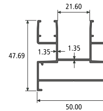
2 TRACK LIGHT SECTION NO. : 914643 Weight / Mtr : 0.865
