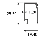
DGU CLIP SECTION NO. : 914641 Weight / Mtr : 0.230
