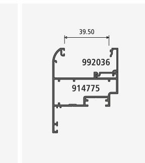
DGU CLIP SECTION NO. : 992036 Weight / Mtr : 0.193
