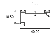
DOOR-BOTTOM-ADAPTOR SECTION NO. : 817918 Weight / Mtr : 0.305
