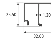
SGU CLIP SECTION NO. : 914549 Weight / Mtr : 0.305
