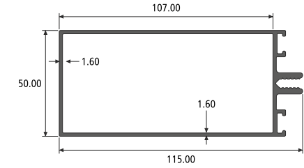
TRANSOM SECTION NO. : 551037 Weight / Mtr : 1.596
