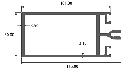
MULLION SECTION NO. : 551038 Weight / Mtr : 2.505
