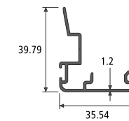
INTERLOCK SECTION NO. : 955391 Weight / Mtr : 0.370
