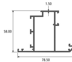
OUTSIDE OP. SHUTTER SECTION NO. : 914353 Weight / Mtr : 1.138
