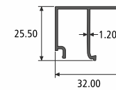
SGU CLIP SECTION NO. : 914549 Weight / Mtr : 0.305
