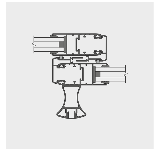
37mm SHUTTER WITH REINFORCEMENT
