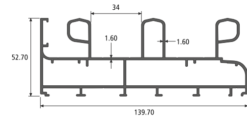
3 TRACK WITH LEG SECTION NO. : 967067 Weight / Mtr : 2.675
