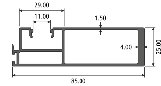
SLEEK REINFORCEMENT INTERLOCK SECTION NO. : 812858 Weight / Mtr : 1.184
